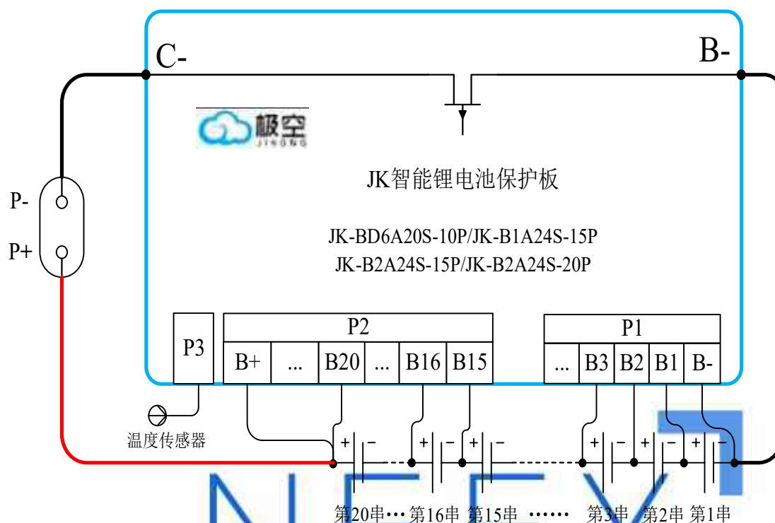
Figure 8. 20 series battery wiring diagram
